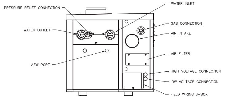
Fig. 2: Component Locations – Left Side
