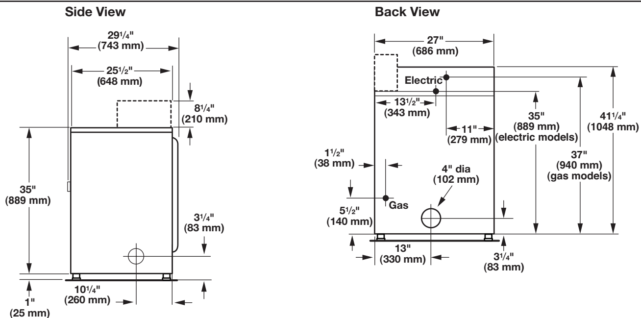
Bottom Exhaust
