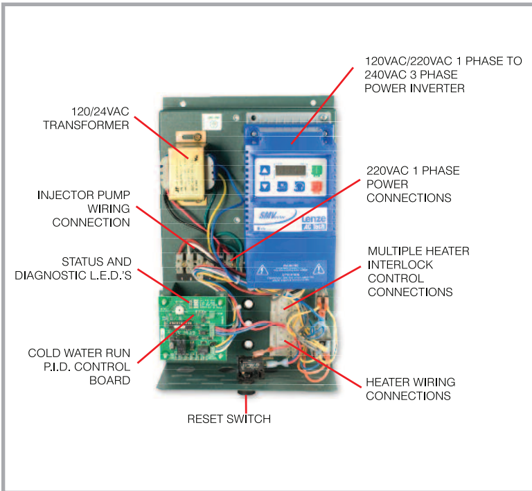
Cold Water Run J-Box Assembly
